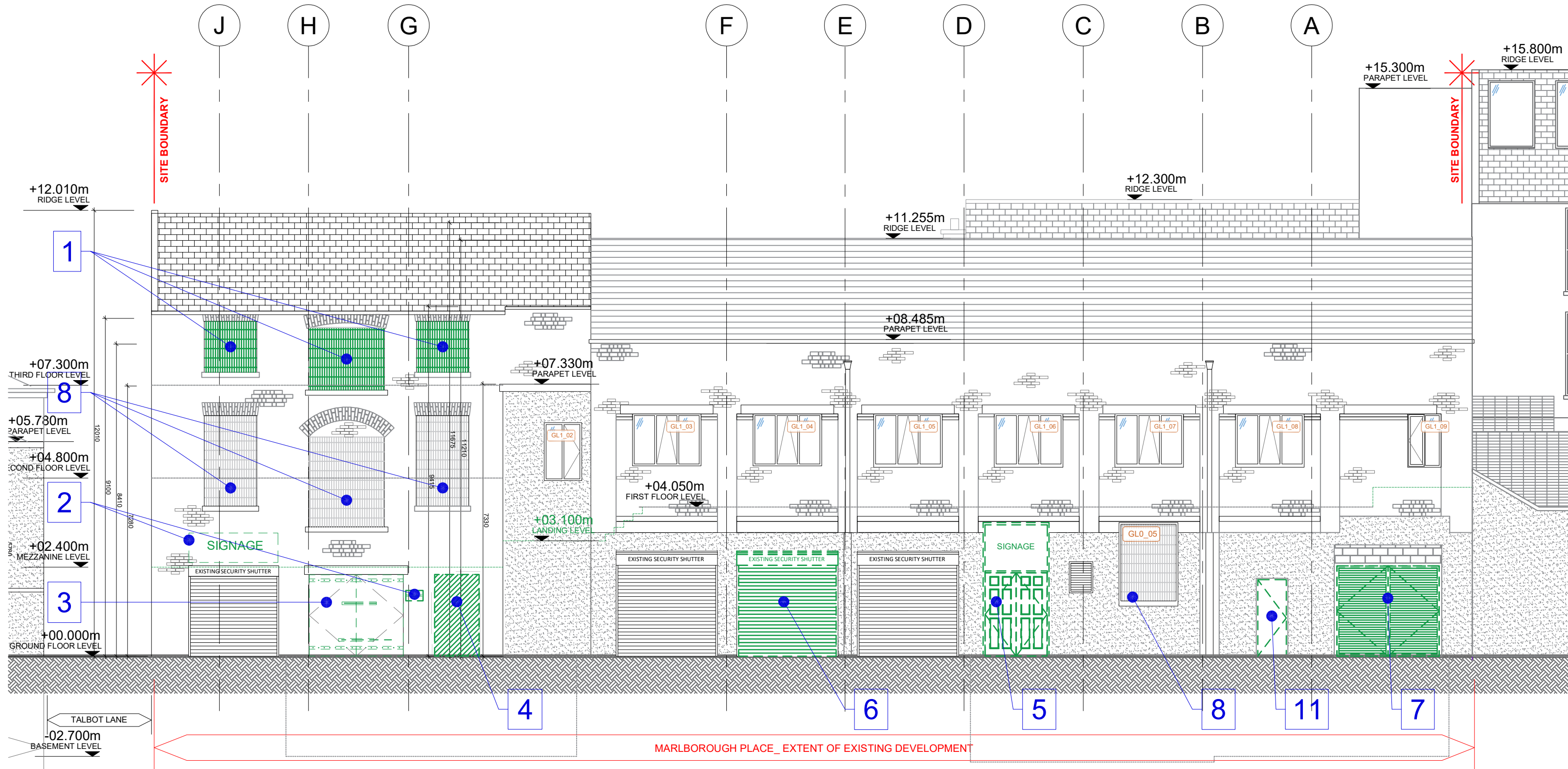
2 30.00 SOUTH ELEVATION_MARLBOROUGH PLACE SCALE: 1:100
