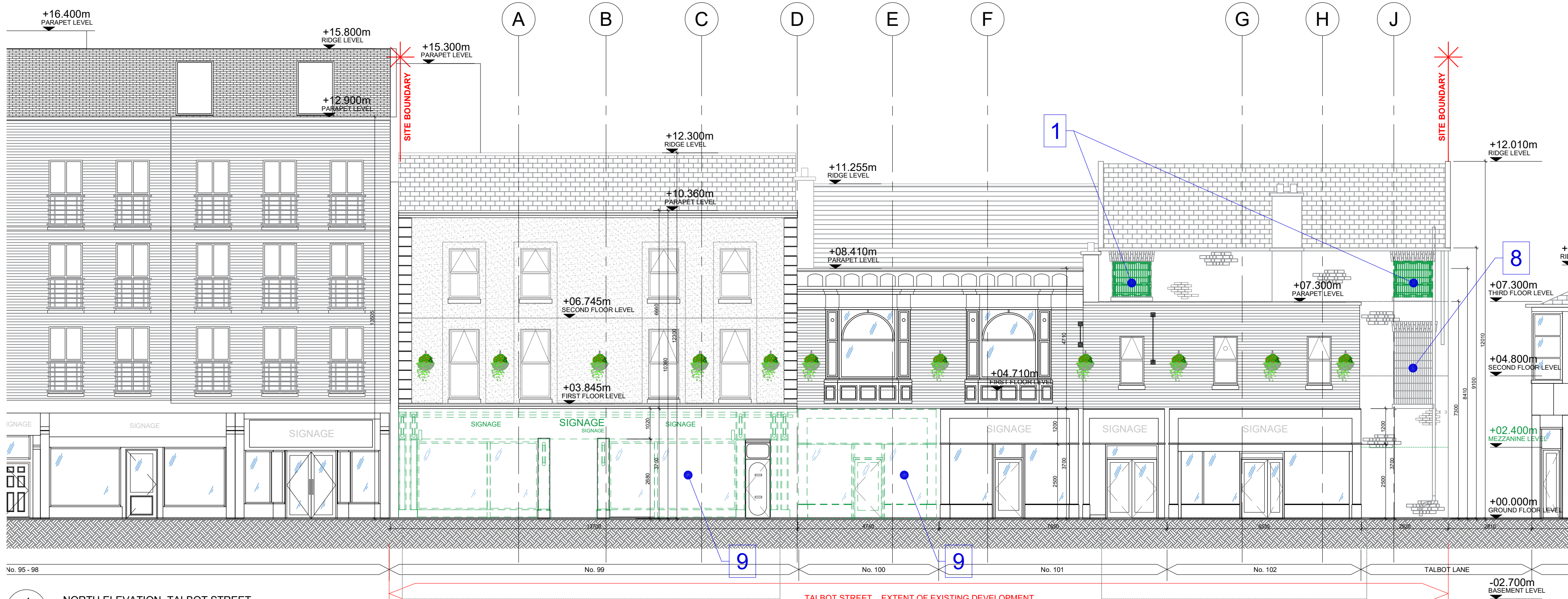
4 30.00 NORTH ELEVATION_TALBOT STREET SCALE: 1:100
